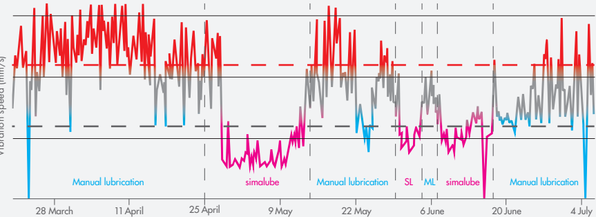
Manual lubrication until the end of April: many upward outliers (red peaks) Automatic lubrication from the end of April: significant harmonisation (pink peaks)
